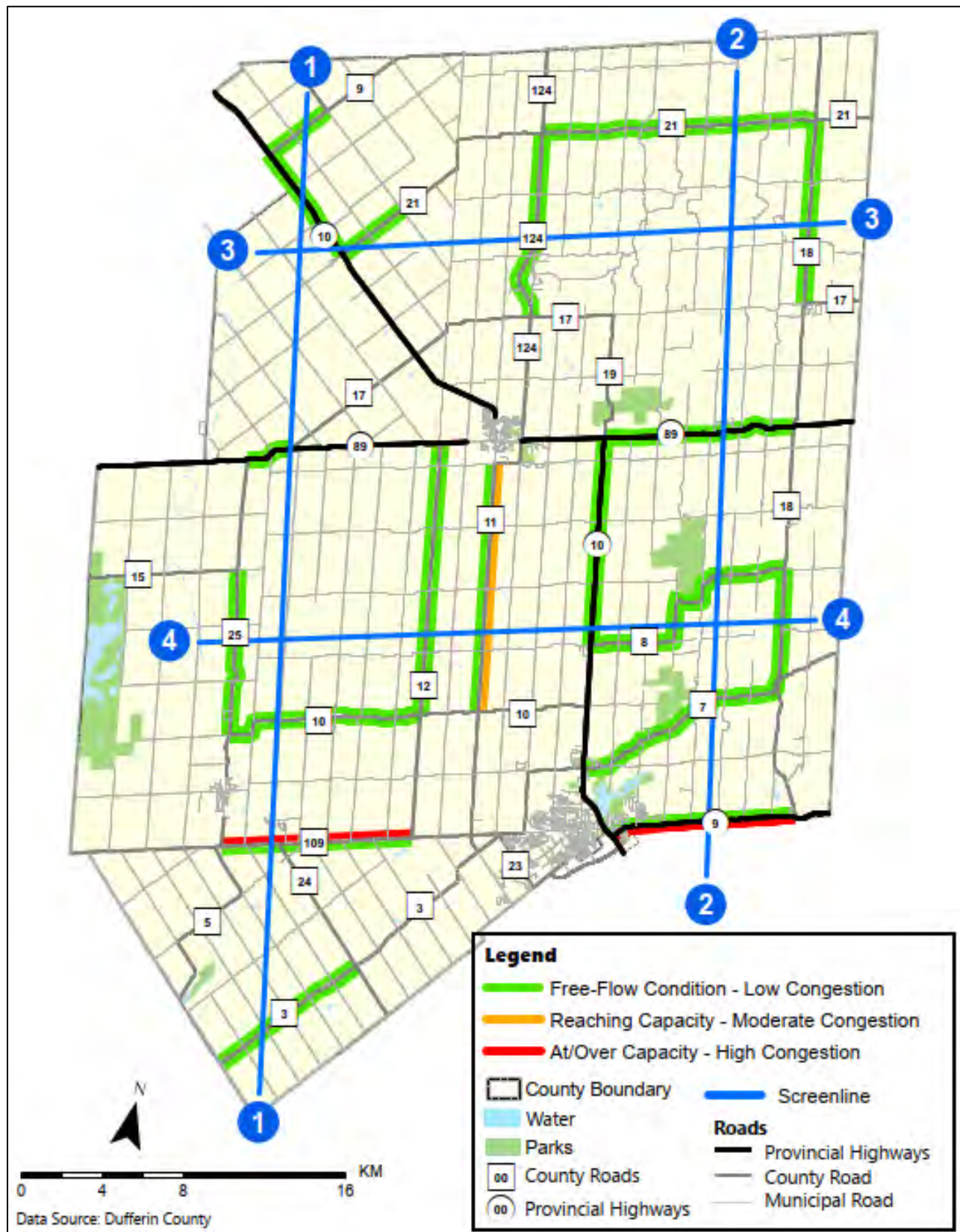
Figure 28. Countywide AM Peak Hour Year 2051 Network Performance
