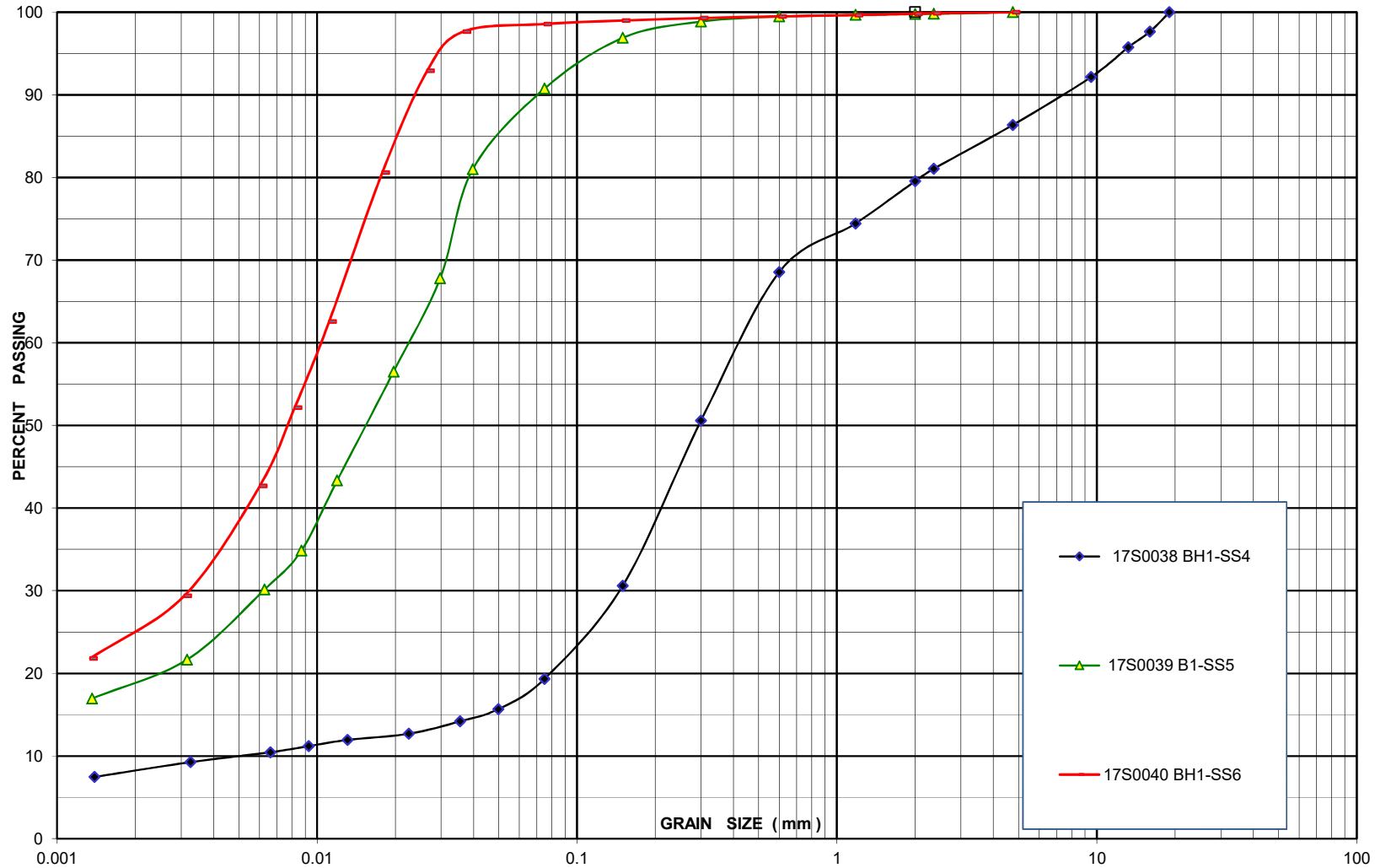
GRAIN SIZE DISTRIBUTION
